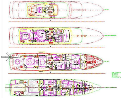
Plan profile
