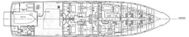
Deck Plan Main
