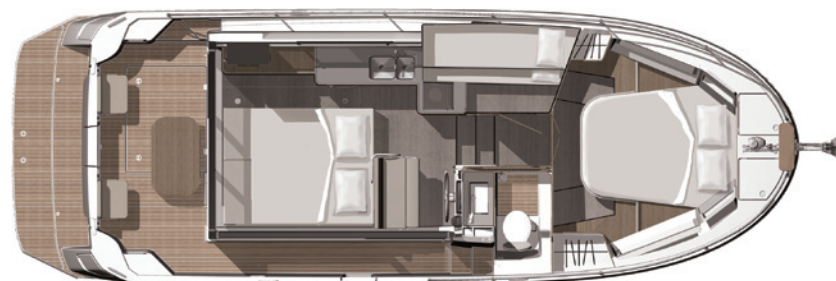
LOWER DECK 2 Cabins version | Version 2 cabines
