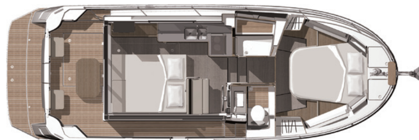
LOWER DECK 1 Cabin version | Version 1 cabine
